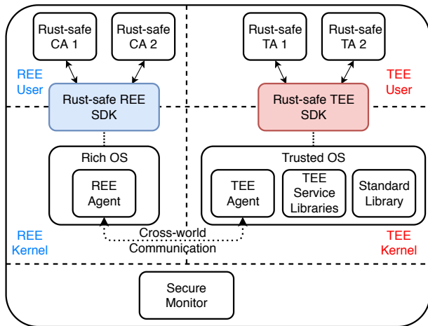
Figure 2: RusTEE Architecture
